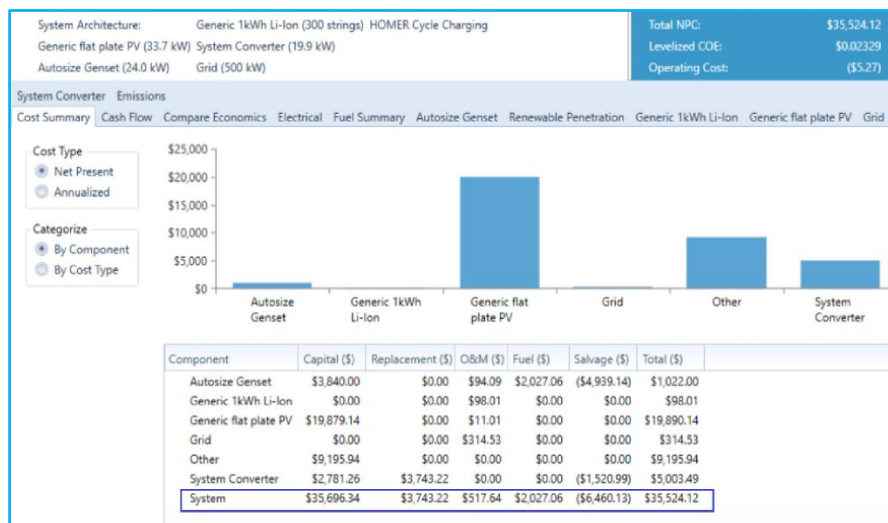
Figure 6. Cost summary.
