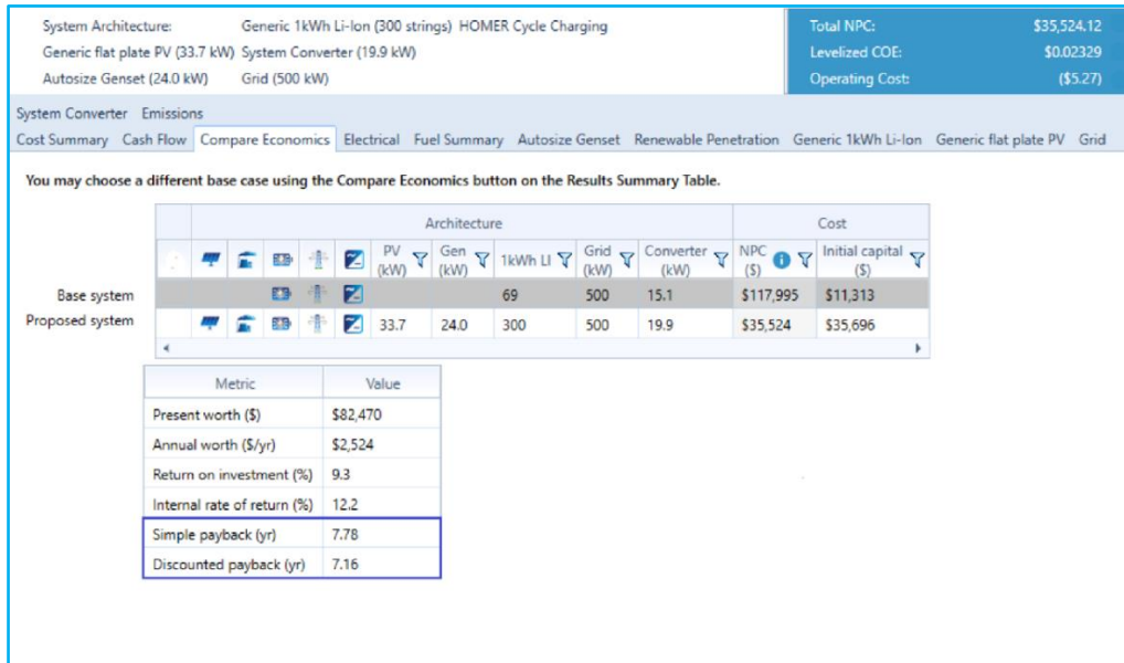
Figure 7. Compare economics.
