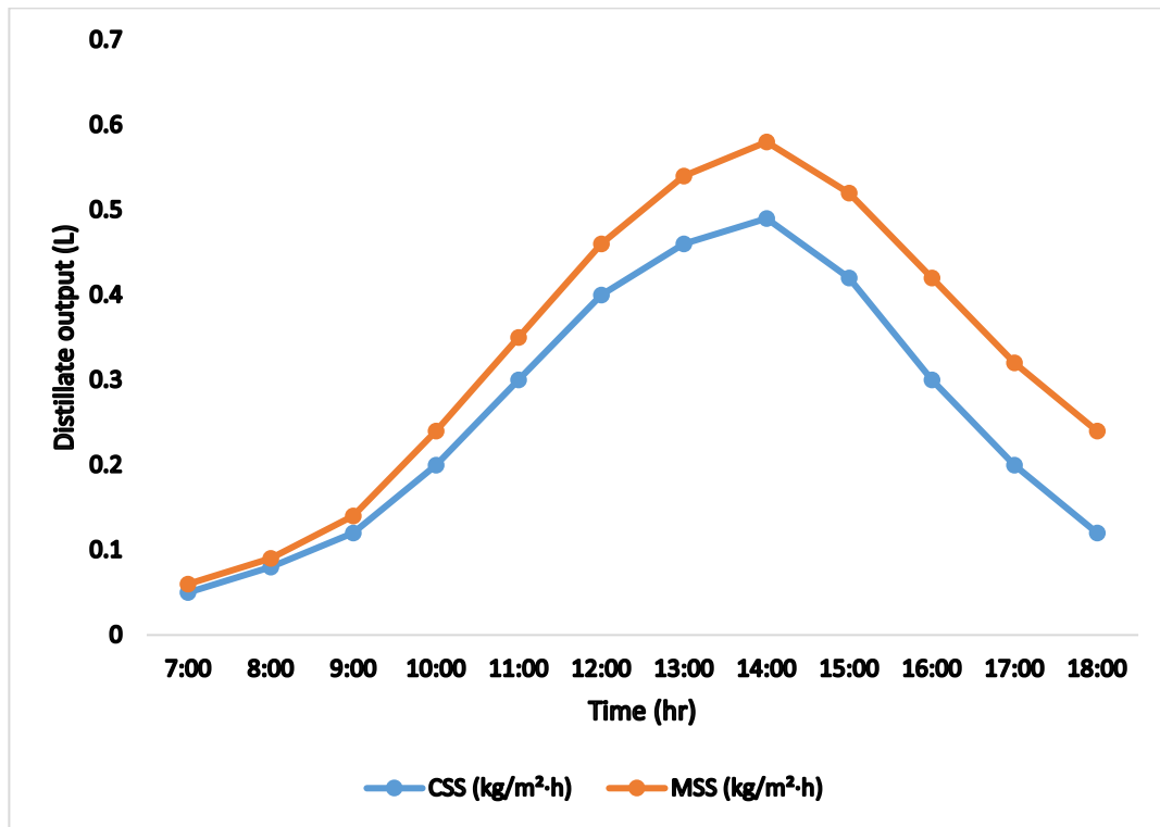
Figure 5. Variations of hourly distillate output vs time (11/04/2025).
